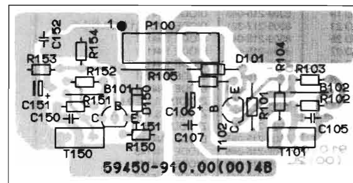
Reglerplatte / Regulator Board V 1000 DPL
